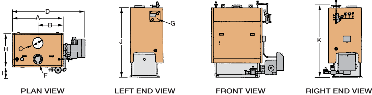
PLAN VIEW
